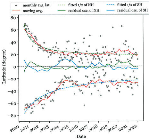
Figure 7. Detrended residual oscillation curves of the monthly averaged latitudes of the coronal jets, separately for the northern and southern hemispheres. Detrending was performed using a 1/x function. The coloring is similar to that shown in Figure 5, with the difference that the green color is for the northern hemisphere and the blue color is for the southern hemisphere jets.
