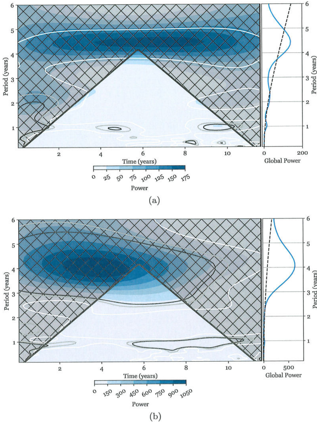
Figure 8. Wavelet analysis of the detrended residual oscillation curves of the monthly averaged latitudes of the coronal jets, separately for the hemispheres. The coloring is similar to that shown in Figure 6. (a) Shows the wavelet analysis of the detrended residual oscillation curve by 1/x of the monthly averaged latitudes of the northern jets. (b) Similarly for the southern jets.
